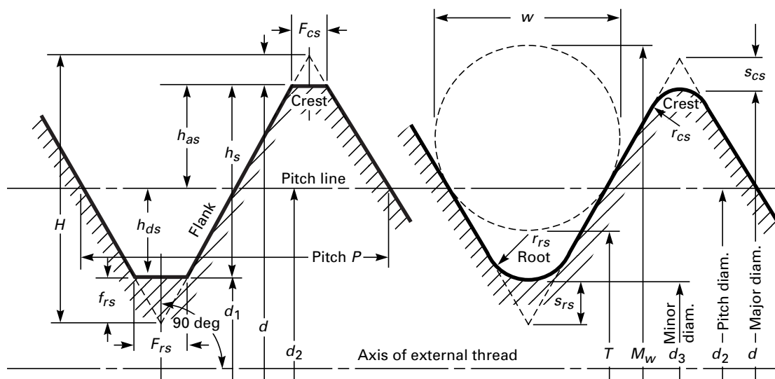
External Thread
