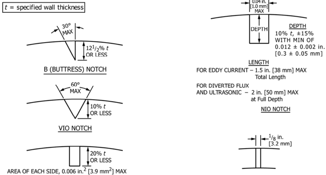
FIG. 1 Calibration Standards
